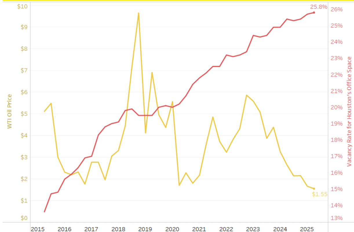
WTI Oil Price and Houston Office Vacancy Rate Quarterly from Q1 2015 to Q1 2025
